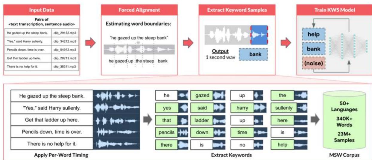
Figure 18.9. A detailed overview of the Multilingual Spoken Words Corpus (MSWC) data processing pipeline: from raw audio and text data input, through forced alignment for word boundary estimation, to keyword extraction and model training.
