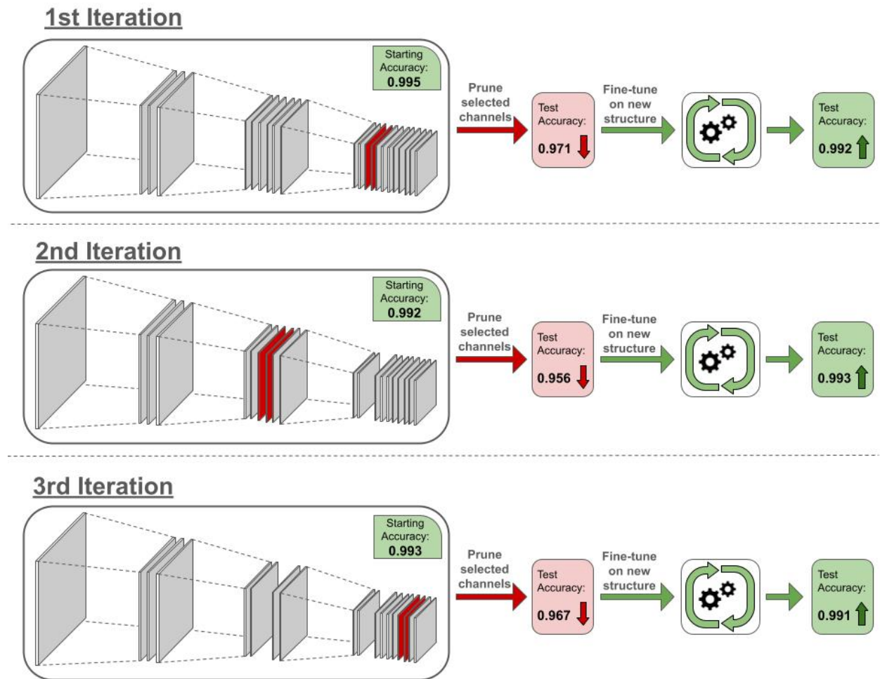
Figure 34.4. In structured iterative pruning, we gradually remove a small set of structures (channels, in this case). Running fine-tuning on the new structure on every iteration allows the model to quickly adapt to the changes. The gradual and controlled nature of iterative pruning ensures that the accuracy drop on each iteration is minimal. Subsequently, the network typically manages to restore its accuracy to levels comparable to its original, unpruned state.
