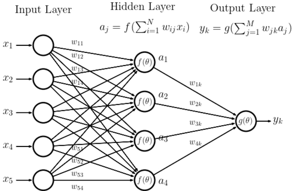
Figure 26.2. Neural Network Diagram: Neural networks consist of alternating linear and nonlinear layers. Linear layers represent the interaction between the outputs of the prior layer and learned weights.
