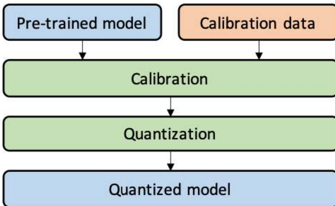
Figure 34.27. In PTQ, a pretrained model is calibrated using calibration data (e.g., a small subset of training data) to compute the clipping ranges and scaling factors (Gholami et al. (2021)).
