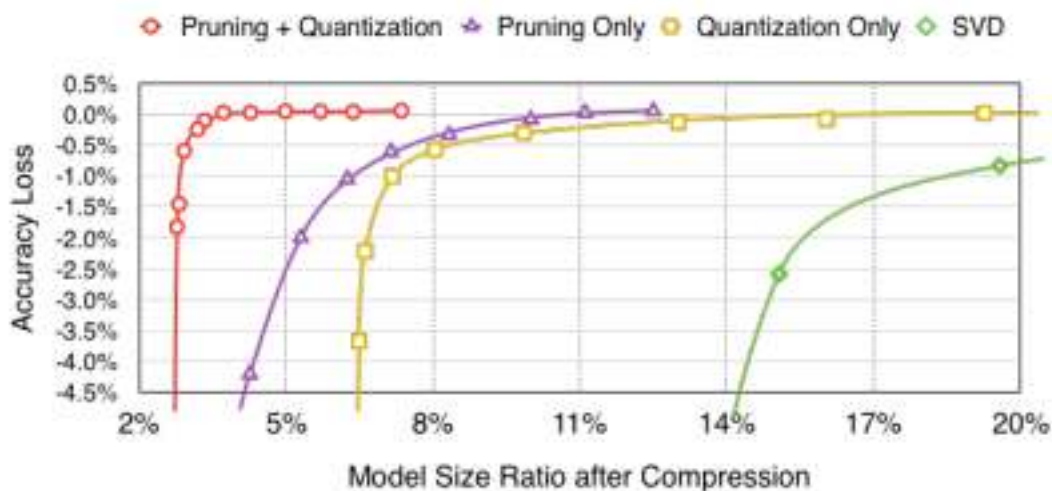
Figure 34.35. Accuracy v.s. compression rate under different compression methods. Pruning and quantization works best when combined (Han, Mao, and Dally (2015)).
