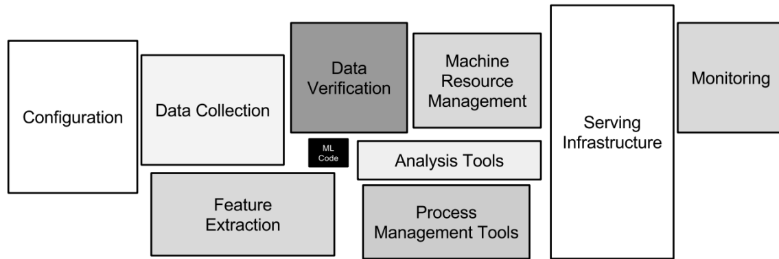
Figure 50.3. ML system components. Credit: Sambasivan et al. (2021a)
