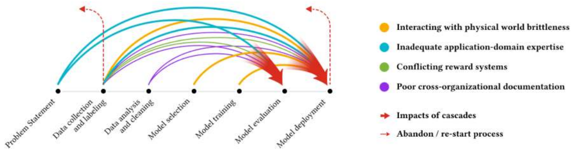
Figure 50.4. Figure 14.3: The flowchart depicts the concept of correction cascades in the ML workflow, from problem statement to model deployment. The arcs represent the potential iterative corrections needed at each stage of the workflow, with different colors corresponding to distinct issues such as interacting with physical world brittleness, inadequate application-domain expertise, conflicting reward systems, and poor cross-organizational documentation. The red arrows indicate the impact of cascades, which can lead to significant revisions in the model development process, while the dotted red line represents the drastic measure of abandoning the process to restart. This visual emphasizes the complex, interconnected nature of ML system development and the importance of addressing these issues early in the development cycle to mitigate their amplifying effects downstream. (Sambasivan et al. 2021a)
