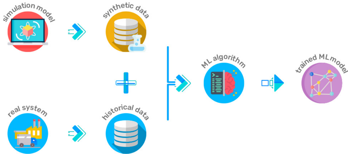
Figure 18.6. Enhancing real-world data with additional synthetic data for training data-hungry ML models (Source: AnyLogic)
