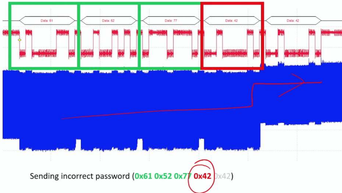
Figure 54.5. Power analysis of an encryption device with a (partially) wrong password. Credit: Colin O'Flynn.
