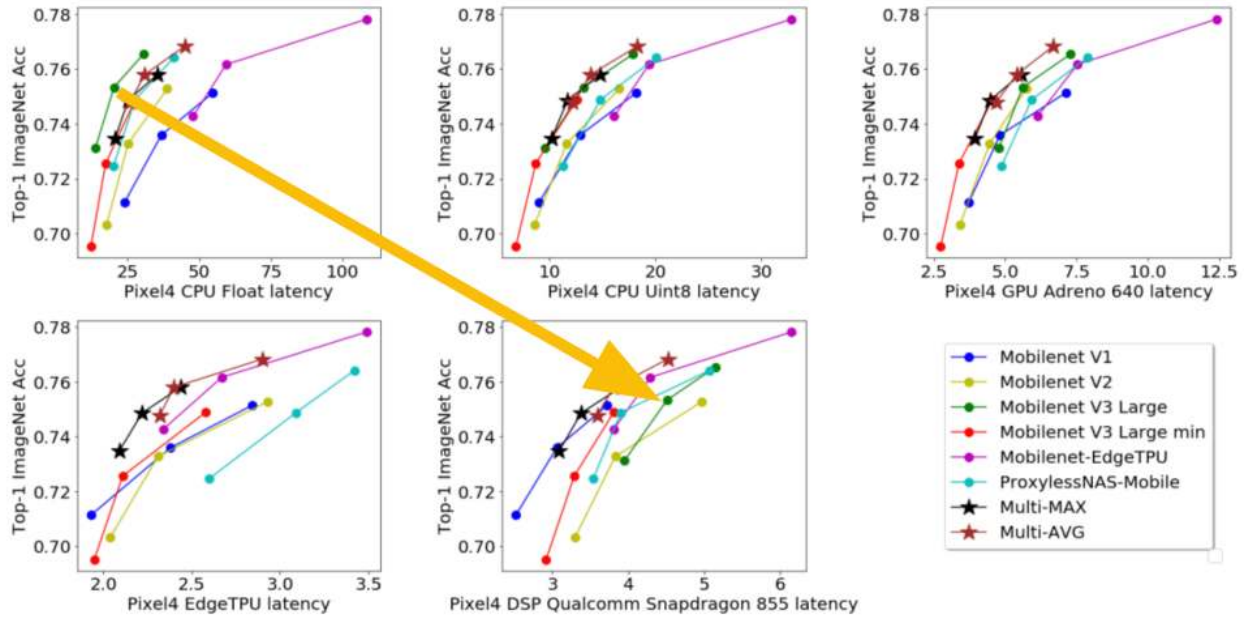
Figure 42.3. Hardware Lottery.
