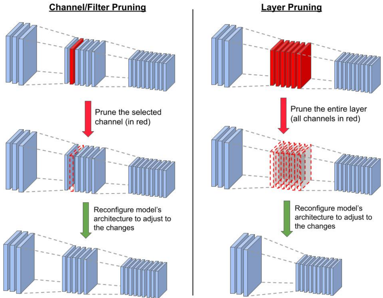
Figure 34.3. On the left, we have an example of a channel-pruning process, in which we remove a specific channel (or filter which subsequently removes the corresponding channel). On the right, we show the process of layer pruning, which involves removing/bypassing an entire layer. Both processes require post-pruning reconfiguration and fine-tuning to adapt the model to the structural changes.
