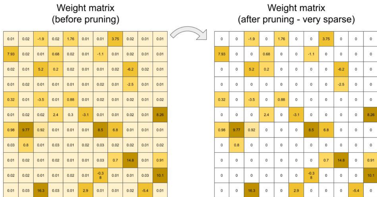
Figure 34.9. Pruning can produce very sparse weight matrices, in which the vast majority of weights are set to zero. While the matrix is now mostly made up of zeros, it still maintains its original shape, which uses up precious memory and introduces calculation inefficiencies.
