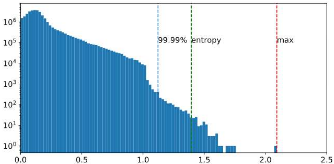
Figure 34.23. Histogram of input activations to layer 3 in ResNet50 and calibrated ranges (Wu, Judd, and Isaev (2020)).
