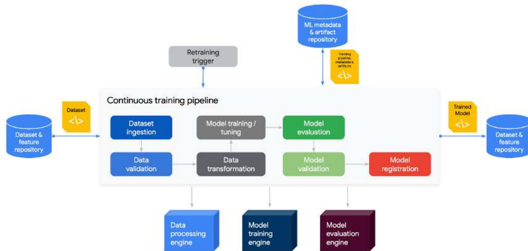
Figure 50.2. MLOps CI/CD diagram. Credit: HarvardX.
