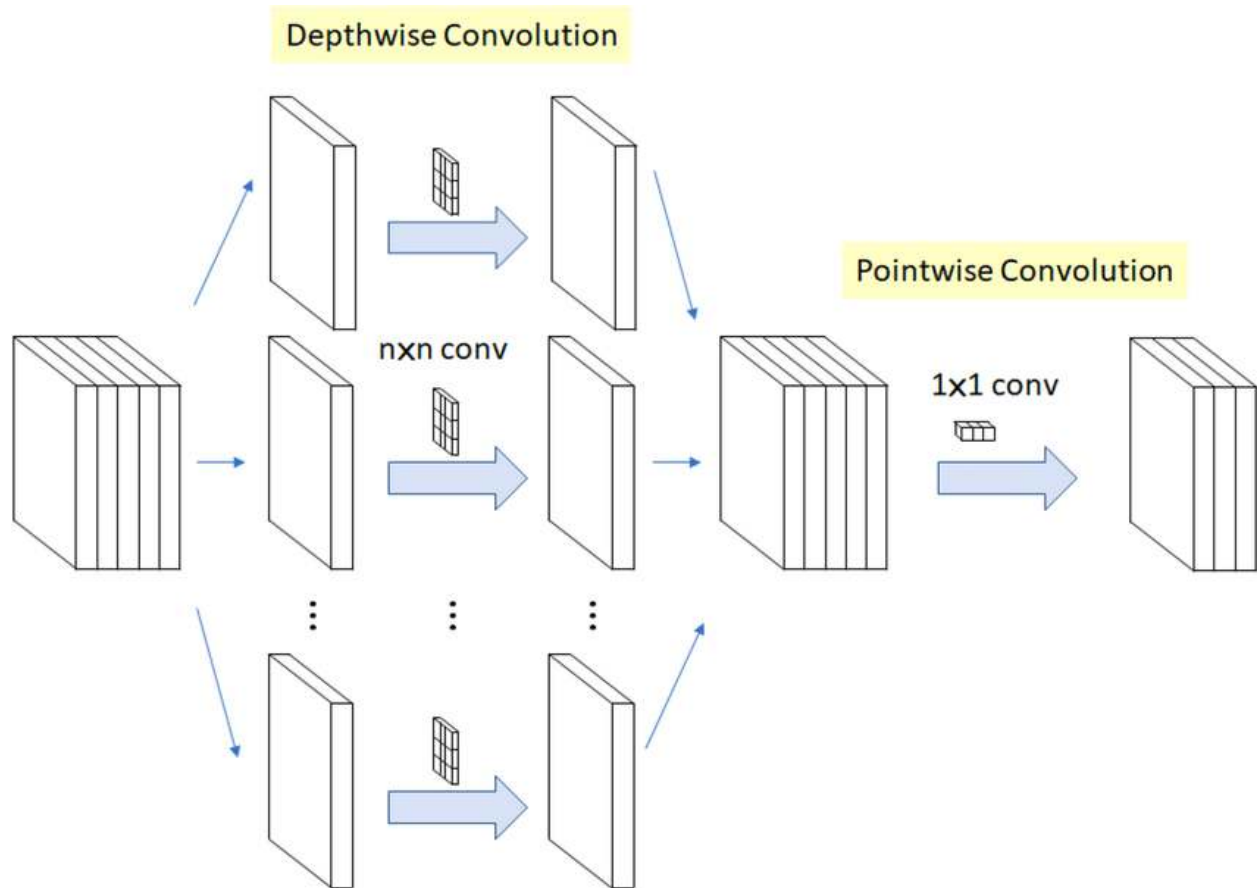
Figure 34.13. A visualization showing each of the individual operations behind a single depthwise separable convolution: first, we give the input image a convolution without modifying the depth. Once those convolutions are completed, we then do a pointwise 1-by-1 convolution to get to the desired number of channels. This reduces the number of parameters, making it a key TinyML technique (Hegde (2023)).
