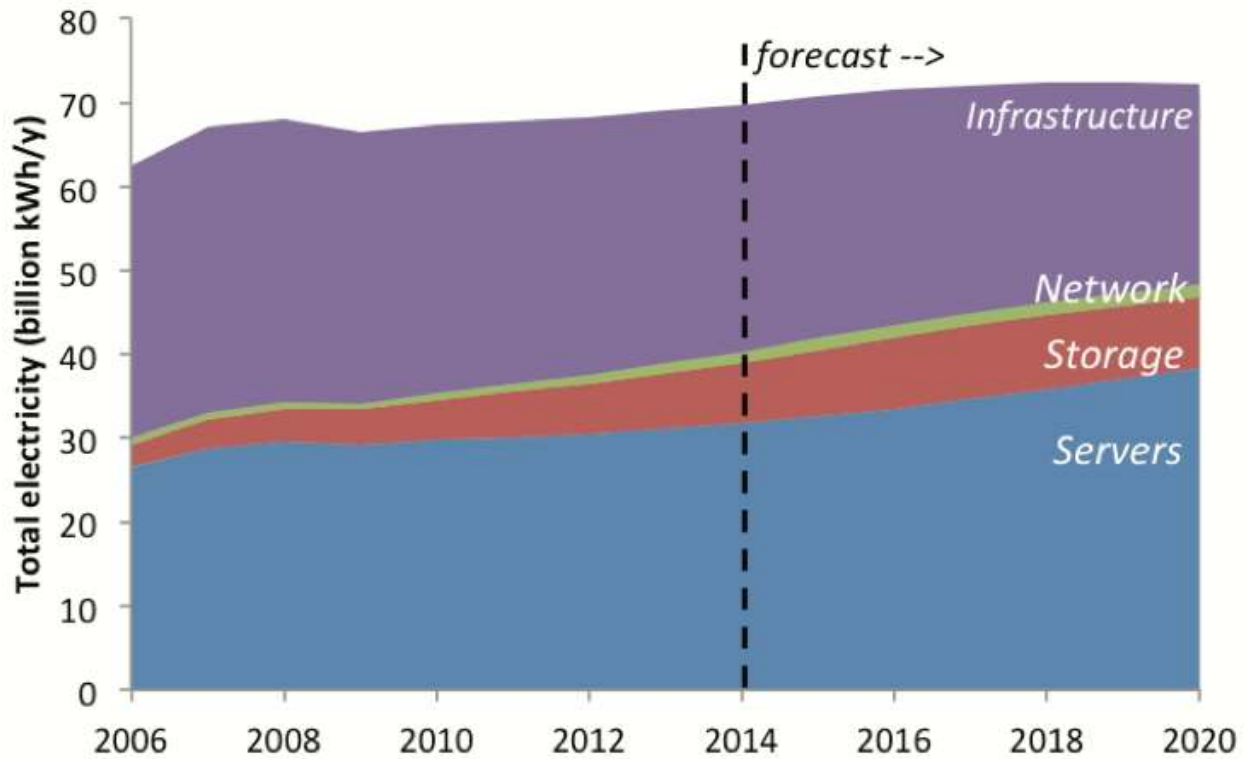
Figure 62.4. Data centers energy consumption in the US. Credit: International Energy Agency (IEA).
