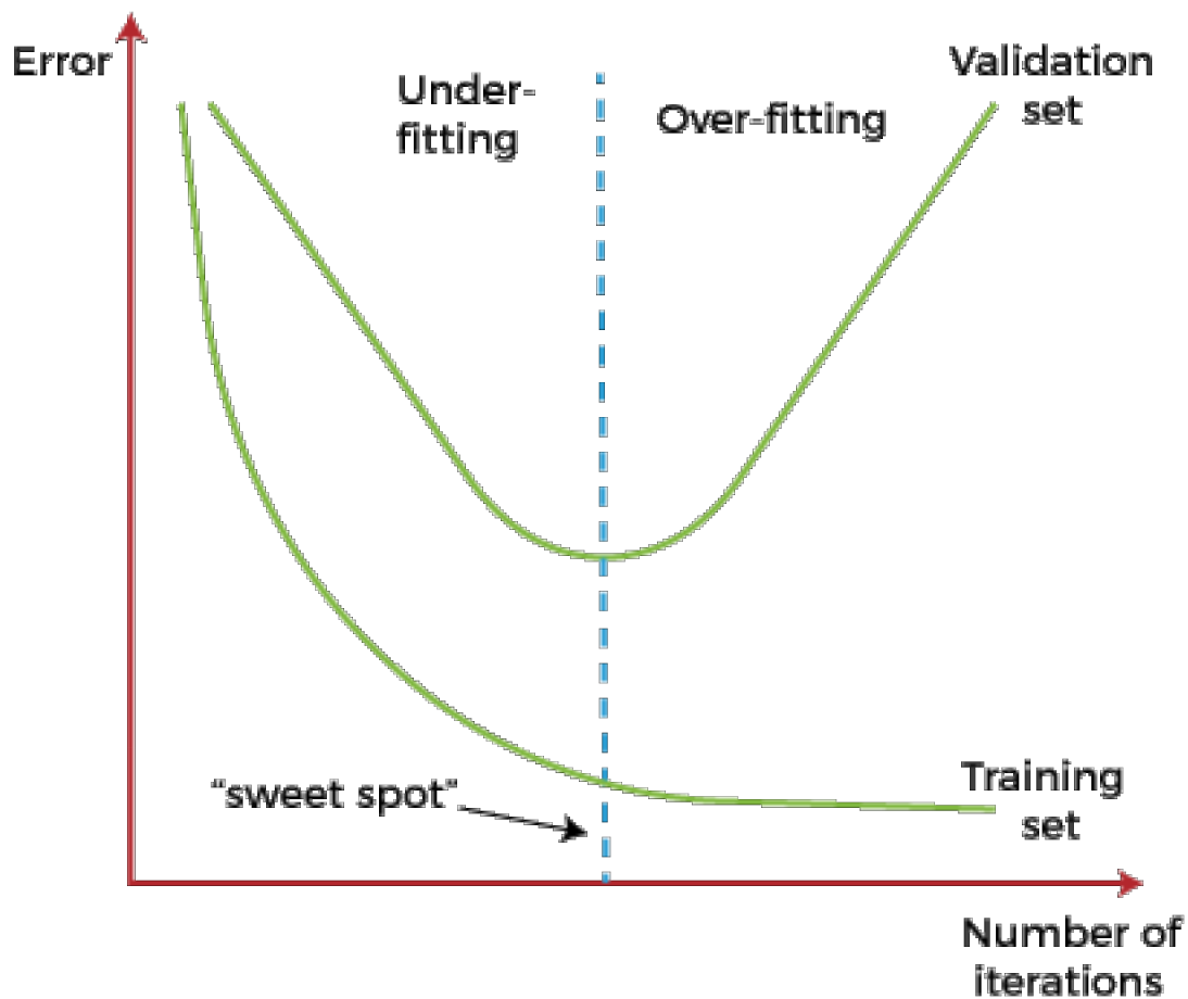
Figure 26.5. Overfitting is one potential problem when training machine learning models, and occurs when the model fits the training data well but fails to generalize to the test data.
