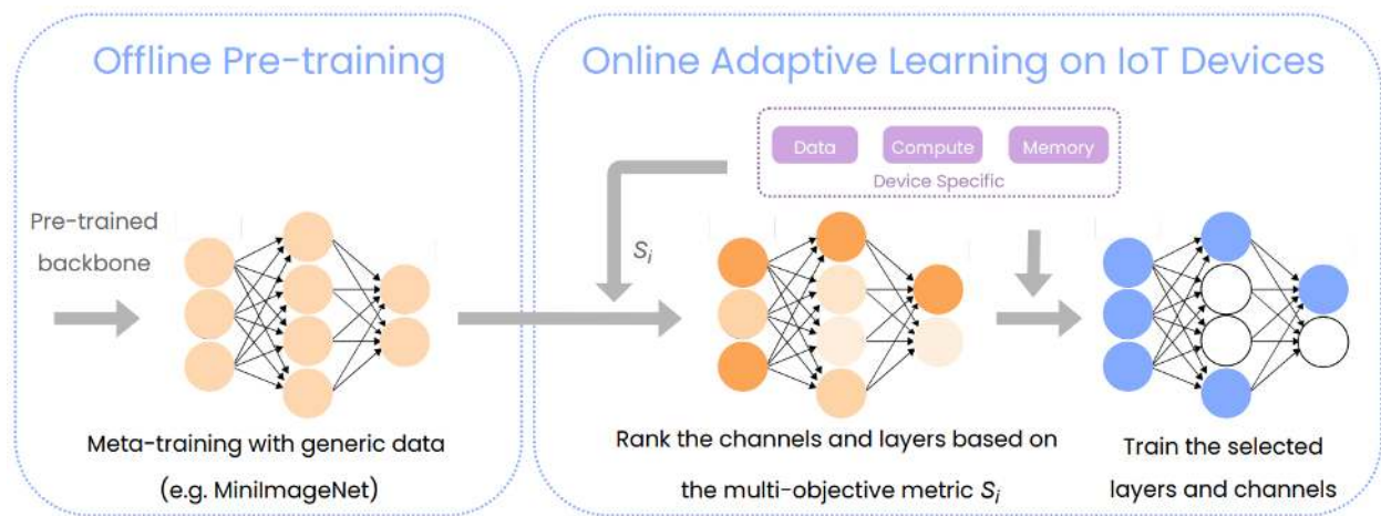
Figure 46.12. TinyTrain workflow. Credit: Y. D. Kwon et al. (2023).
