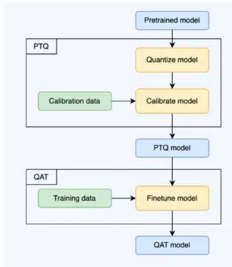
Figure 34.29. Note that QAT is an extension of PTQ. It receives the model quantized by PTQ and re-trains it to finetune quantized parameters (“The Ultimate Guide to Deep Learning Model Quantization and Quantization-Aware Training” (n.d.)).
