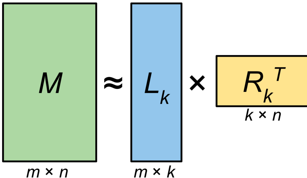
Figure 34.11. A visualization showing the decrease in parameterization enabled by low-rank matrix factorization. Observe how the matrix M can be approximated by the product of matrices L_k and R_k^T . For intuition, most fully connected layers in networks are stored as a projection matrix M , which requires m \times n parameter to be loaded on computation. However, by decomposing and approximating it as the product of two lower rank matrices, we thus only need to store m \times k + k \times n parameters in terms of storage while incurring an additional compute cost of the matrix multiplication. So long as k < n/2 , this factorization has fewer parameters total to store while adding a computation of runtime O(mkn) (Gu (2023)).
