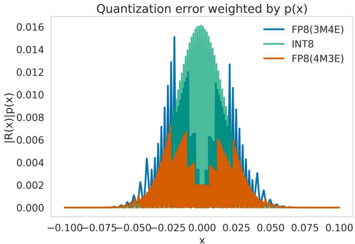
Figure 34.47. A smooth histogram of quantization error. (Kuzmin et al. 2022)
