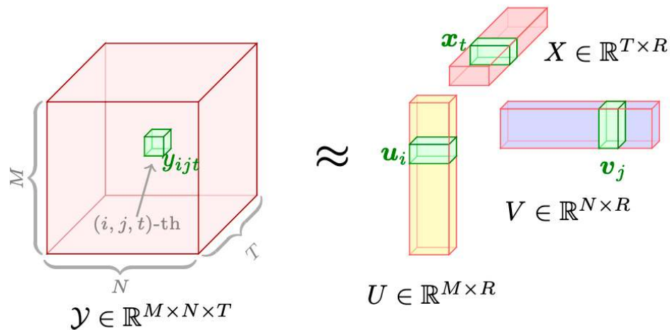
Figure 34.12. A visualization showing the decrease in parameterization enabled by tensor decomposition. Observe how the shown three-dimensional tensor y can be approximated by three matrices, all of lower rank, greatly reducing the number of parameters to be held in memory (Xinyu (n.d.)).
