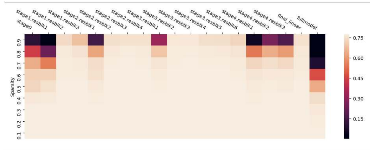
Figure 34.45. A heat map showing a sparse neural network.
