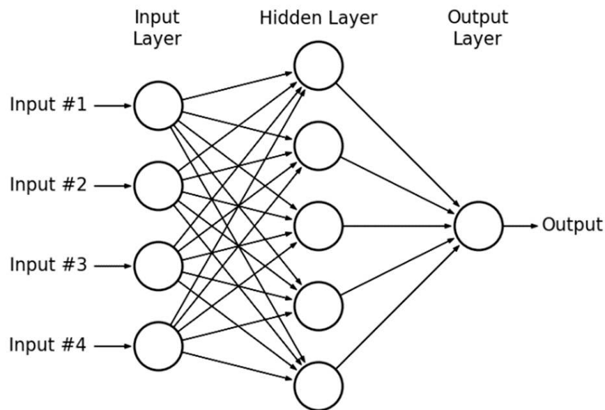
Figure 6.5. Multilayer Perceptron
