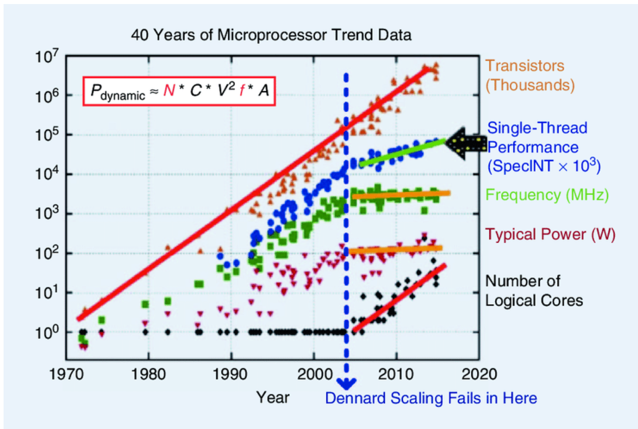
Figure 38.2. Microprocessor trends. Credit: Karl Rupp.
