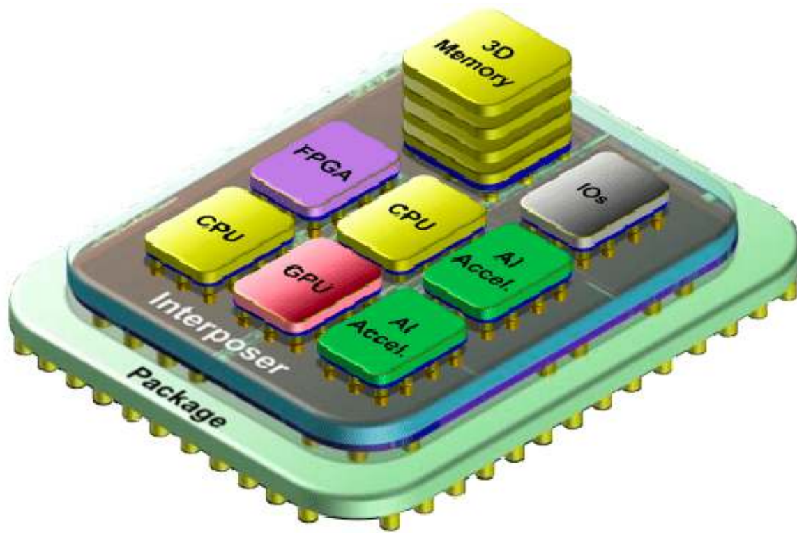
Figure 38.6. Chiplet partitioning. Credit: Vivet et al. (2021).
