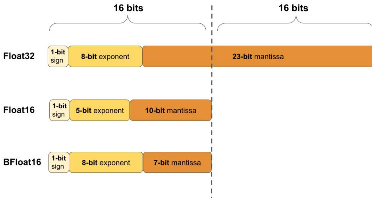
Figure 34.14. Three floating-point formats.
