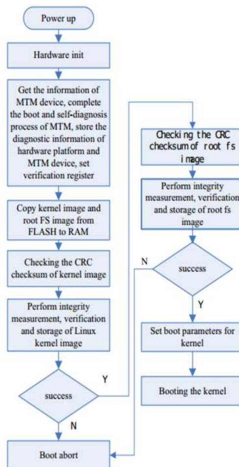
Figure 54.8. Secure Boot flow. Credit: R. V. and A. (2018).
