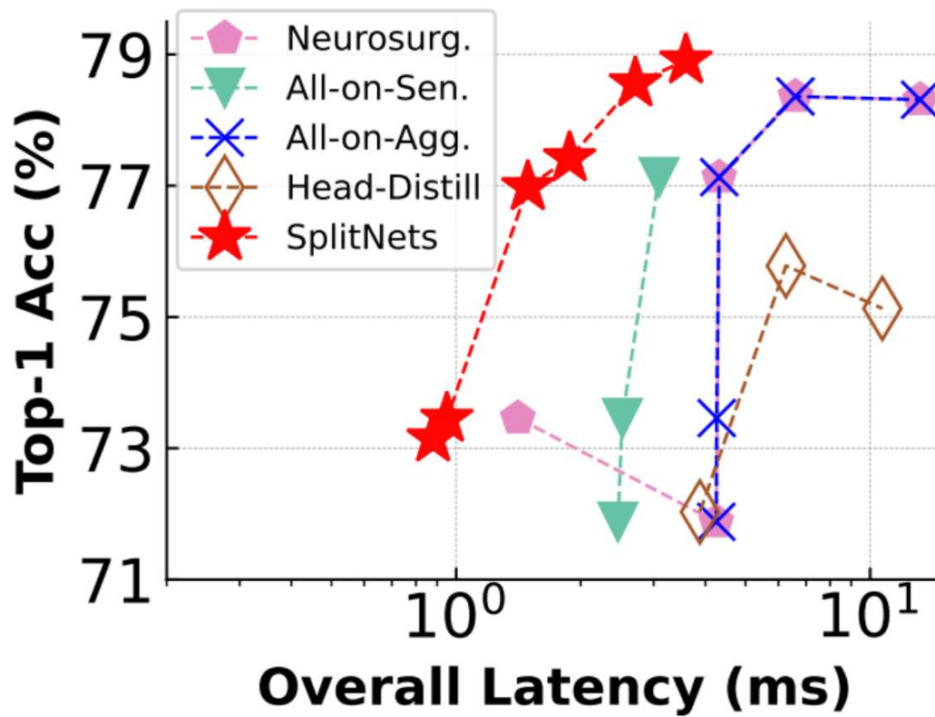
Figure 34.43. A chart showing a comparison between the performance of SplitNets vs all on sensor and all on aggregator approaches. (Dong et al. 2022)
