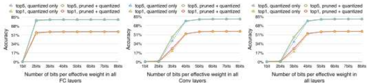
Figure 34.36. Pruning doesn't hurt quantization. Dashed: quantization on unpruned network. Solid: quantization on pruned network; Accuracy begins to drop at the same number of quantization bits whether or not the network has been pruned. Although pruning made the number of parameters less, quantization still works well, or even better (3 bits case on the left figure) as in the unpruned network (Han, Mao, and Dally (2015)).
