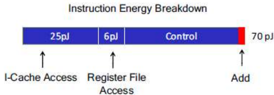
Figure 34.15. Tables comparing energy use by quantized operations (Isscc (2014)).
