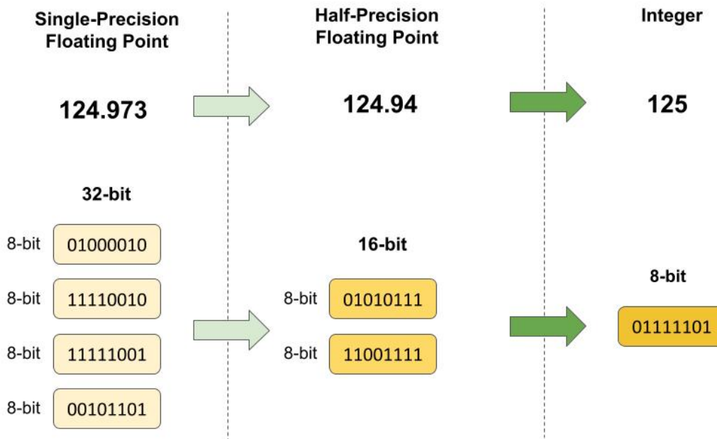
Figure 30.4. One method of quantization involves rounding to the nearest representable number. Quantization helps save on memory while minimizing performance loss.
