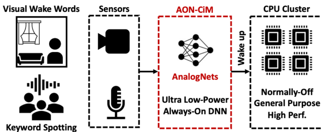
Figure 34.40. A figure showing how Computing in Memory can be used for always-on tasks to offload tasks of the power consuming processing unit (C. Zhou et al. 2021)
