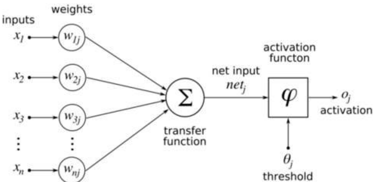
Figure 6.4. Perceptron (source)
