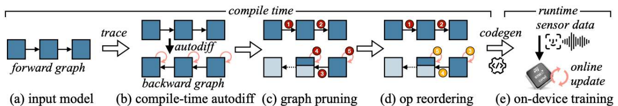
Figure 46.10. TTE workflow.
