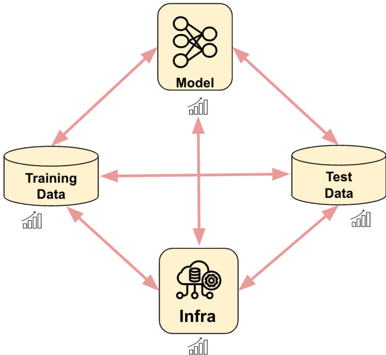
Figure 42.7. Benchmarking trifecta.
