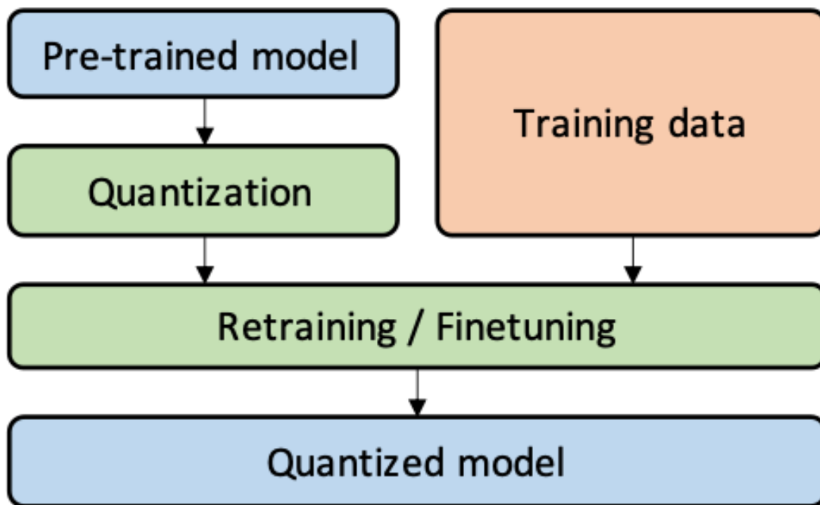
Figure 34.28. In QAT, a pretrained model is quantized and then finetuned using training data to adjust parameters and recover accuracy degradation. Note: the calibration process is often conducted in parallel with the finetuning process for QAT (Gholami et al. (2021)).
