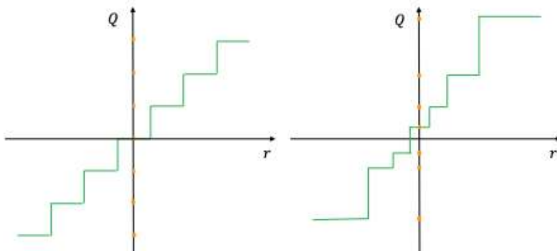
Figure 34.21. Comparison between uniform quantization (left) and non-uniform quantization (right) (Gholami et al. (2021)).
