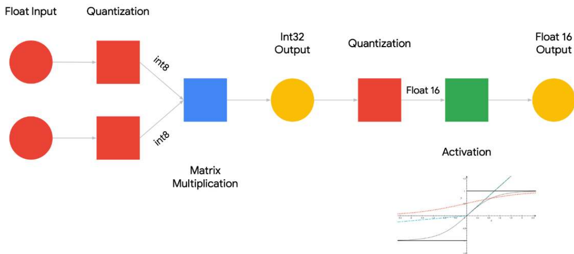
Figure 34.31. Diagram of quantizing weights and activations
