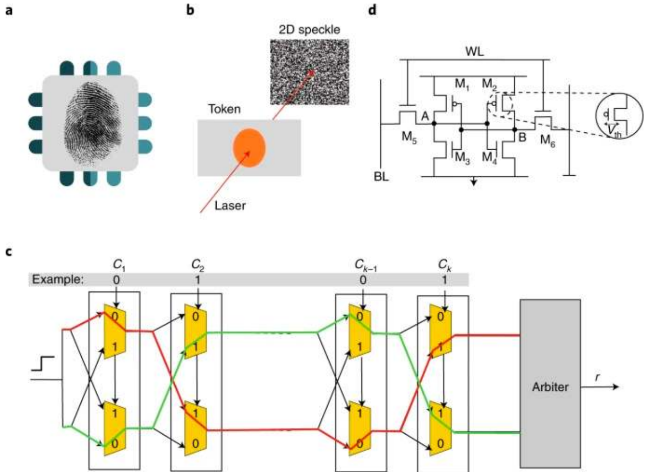
Figure 54.9. PUF basics. Credit: Gao, Al-Sarawi, and Abbott (2020).
