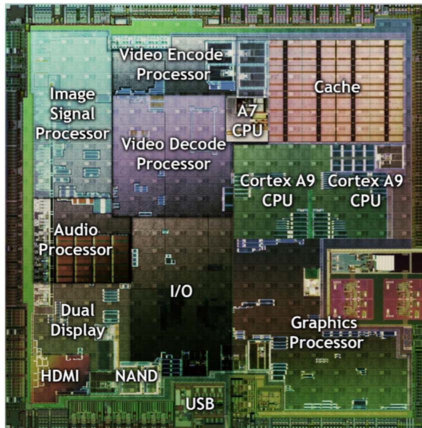
Figure 2.5. NVIDIA's Tegra 2 combines two ARM Cortex-A9 cores with an ARM7 for SoC management tasks.
