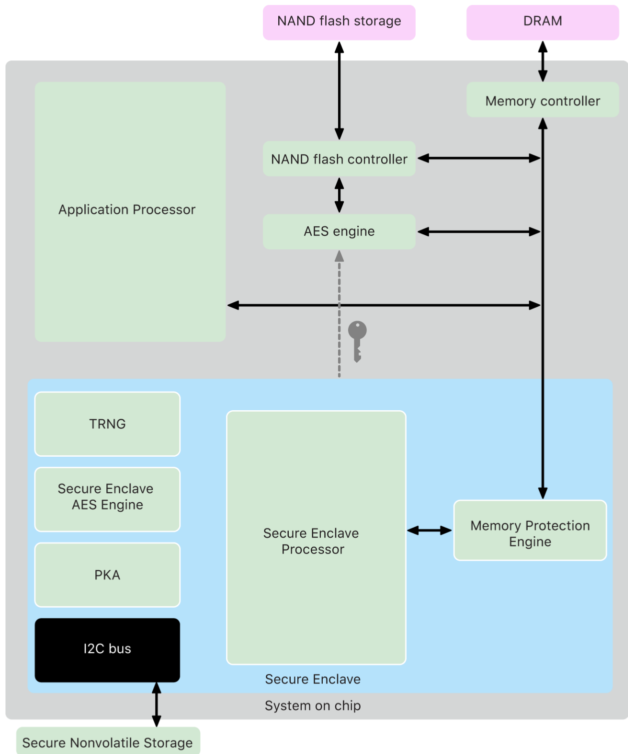
Figure 54.7. System-on-chip secure enclave. Credit: Apple.
