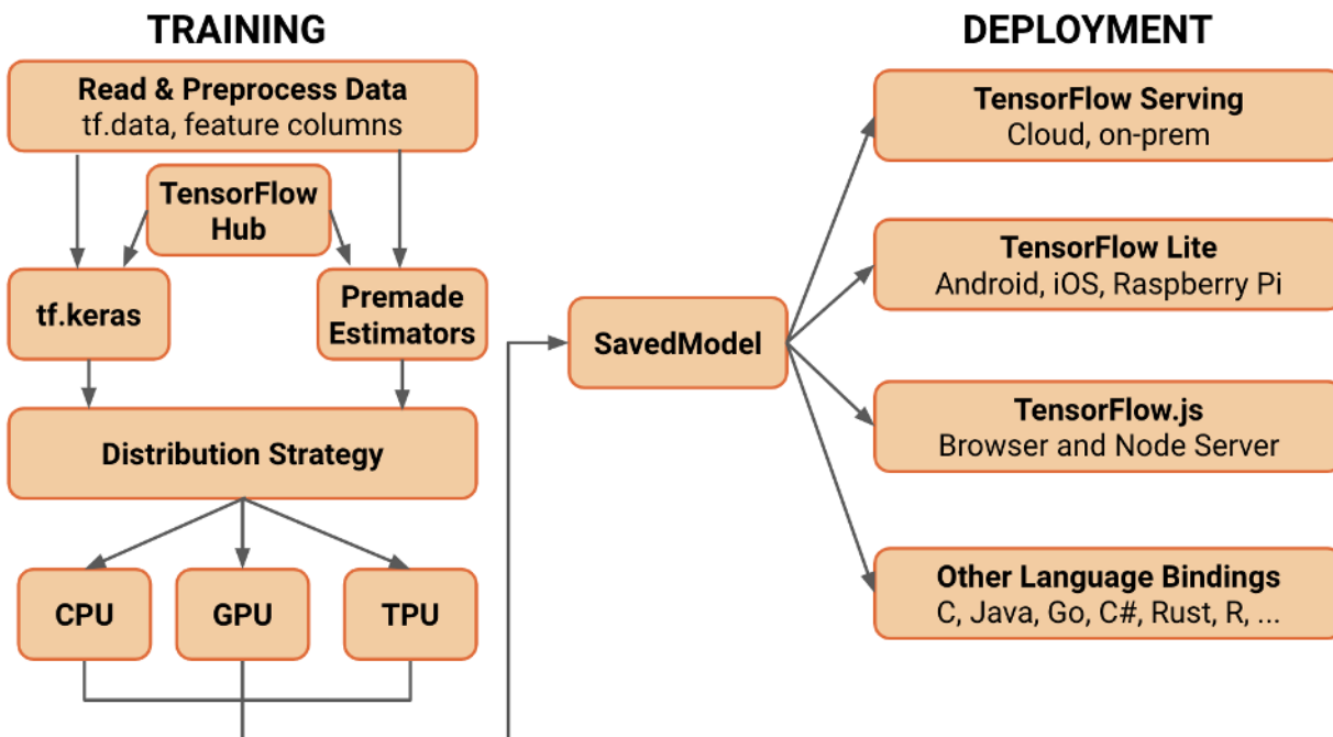
Figure 22.3. Architecture overview of TensorFlow 2.0 (Source: Tensorflow)
