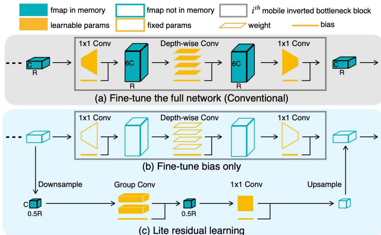
Figure 46.11. TinyTL workflow. Credit: Cai et al. (2020).)
