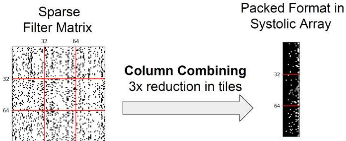
Figure 34.46. A figure showing the sparse columns of the filter matrix of a CNN that are aggregated to create a dense matrix that, leading to smaller dimensions in the matrix and more efficient computations (H. T. Kung, McDanel, and Zhang 2018)
