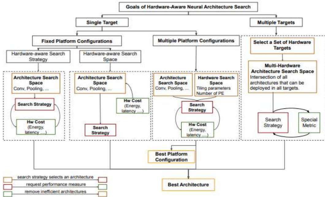
Figure 34.38. Taxonomy of HW-NAS (Benmeziane et al. 2021)
