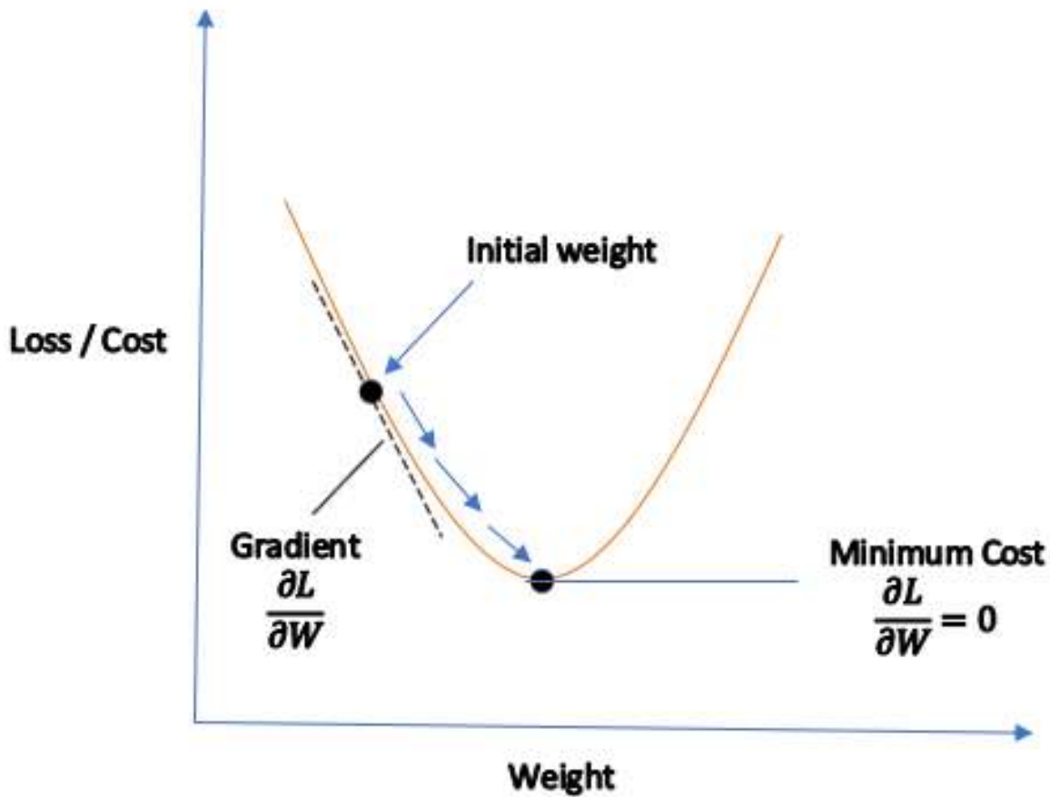
Figure 26.3. Optimizing a neural network involves repeated application of gradient descent. This involves minimizing the loss function, which can be done by repeatedly taking steps in the direction of the gradient of the network with respect the loss function.
