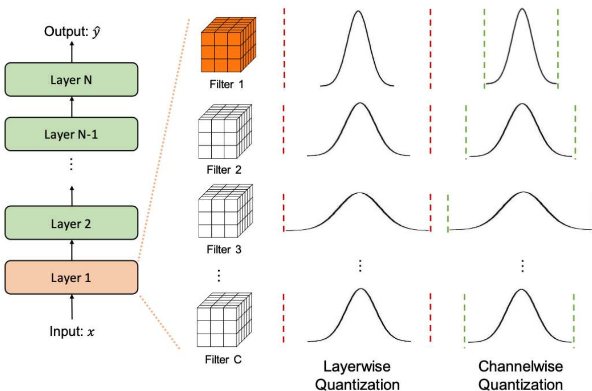
Figure 34.25. Illustration of the main forms of quantization granularities. In layerwise quantization, the same clipping range is applied to all filters which belong to the same layer. Notice how this can result in lower quantization resolutions for channels with narrow distributions, e.g. Filter 1, Filter 2, and Filter C. A higher quantization resolution can be achieved using channelwise quantization which dedicates different clipping ranges to different channels (Gholami et al. (2021)).
