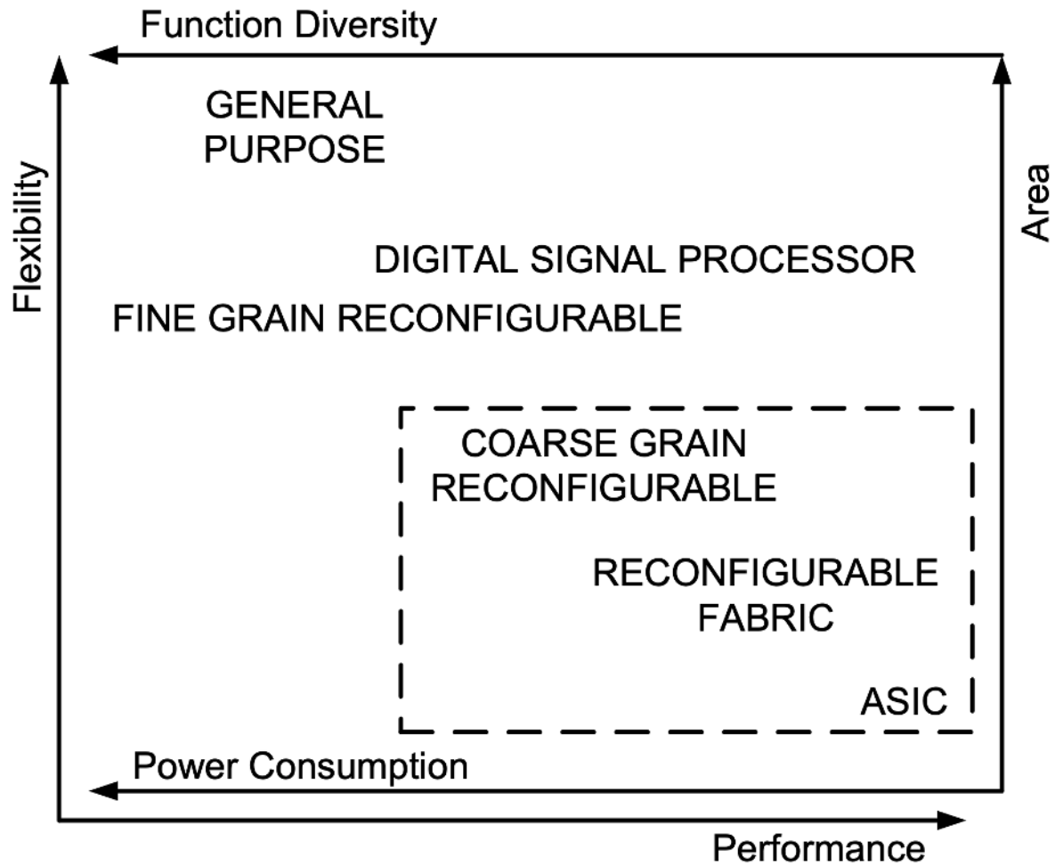
Figure 38.3. Design tradeoffs. Credit: S. Huang, Waeijen, and Corporaal (2022)
