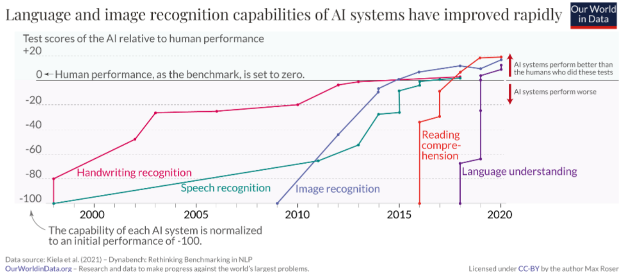
Figure 42.6. AI vs human performance. Credit: Kiela et al. (2021).
