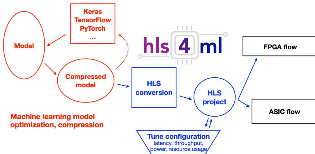
Figure 34.41. A Diagram showing the workflow with the hls4ml framework (Fahim et al. 2021)
