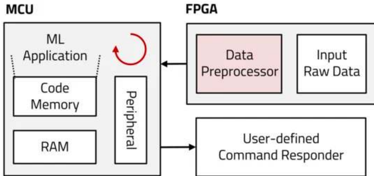
Figure 34.42. A diagram showing how an FPGA was used to offload data preprocessing of the general purpose computation unit. (J. Kwon and Park 2021)
