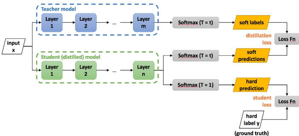
Figure 34.10. A visualization of the training procedure of knowledge distillation. Note how the logits or soft labels of the teacher model are used to provide a distillation loss for the student model to learn from (IntelLabs (2023)).
