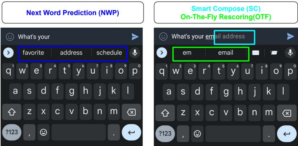
Figure 46.8. Google G Board Features. Credit: Zheng et al., (2023).
