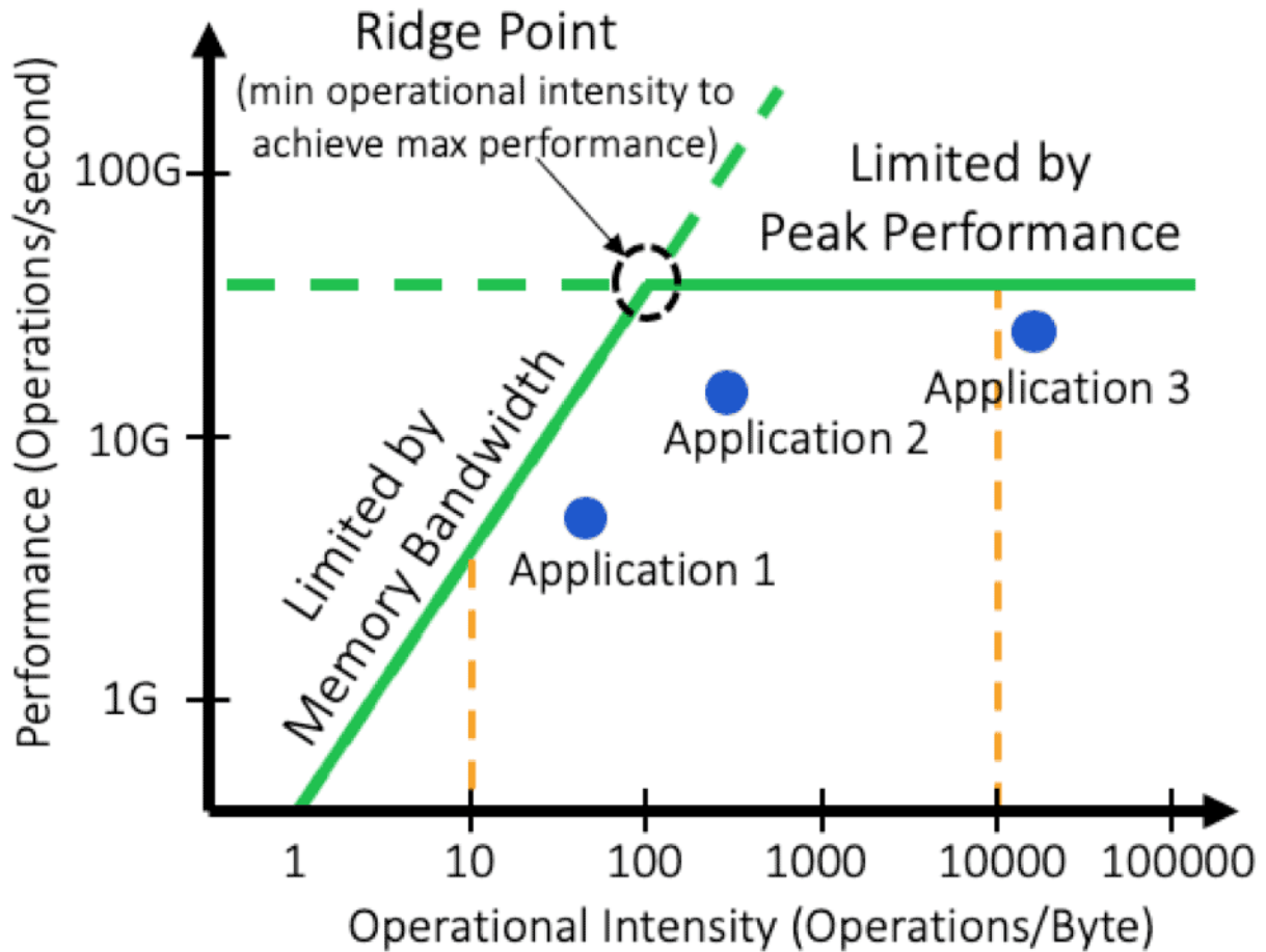
Figure 26.8. AI training is typically compute bound due to the high arithmetic intensity of matrix-multiplication when batch size is large.
