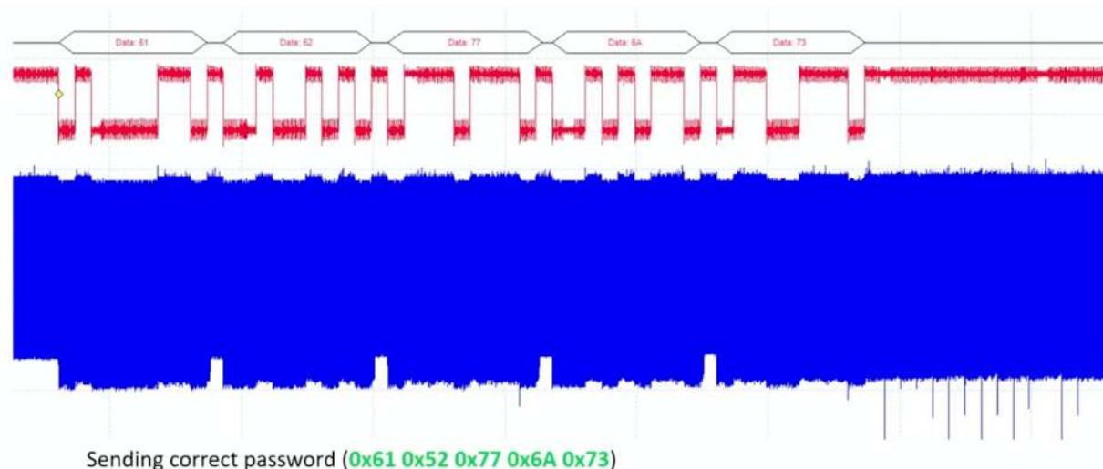
Figure 54.4. Power analysis of an encryption device with a correct password. Credit: Colin O'Flynn.
