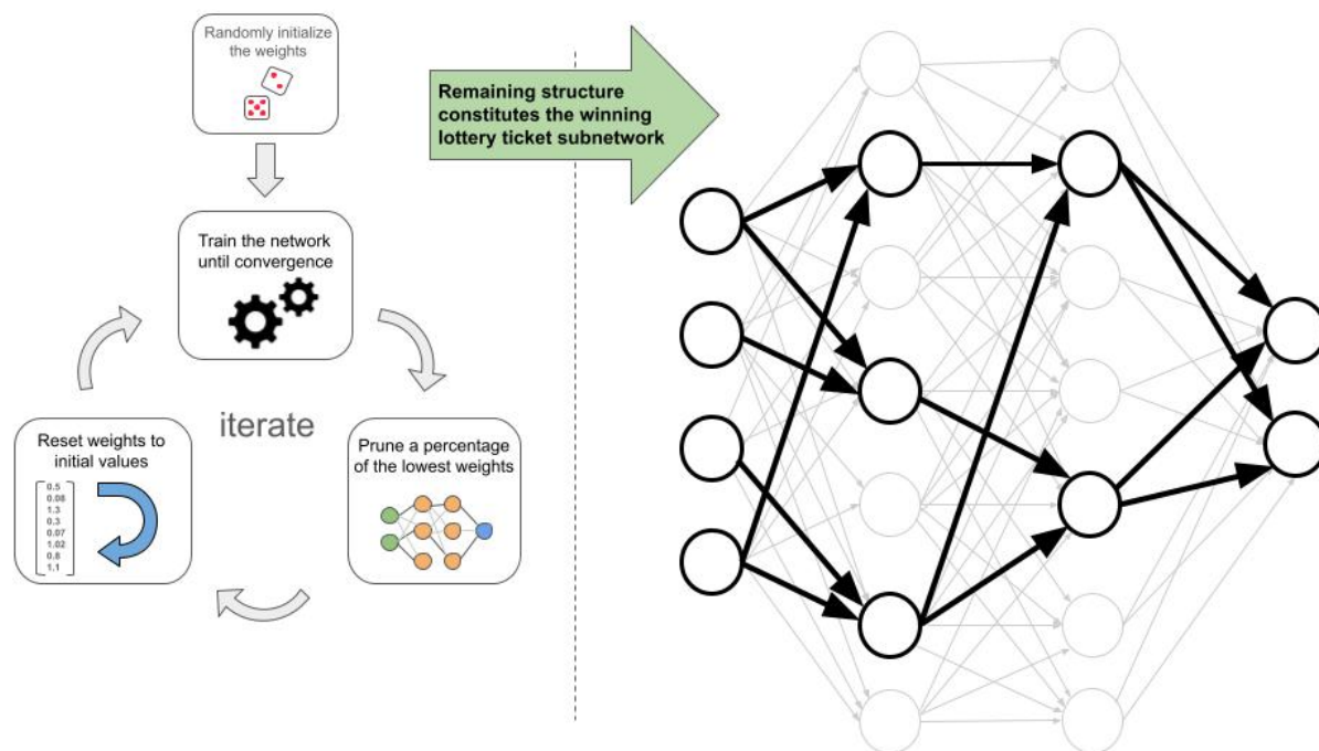
Figure 34.8. On the left, we have a simplified overview of the process of finding the winning ticket subnetwork. On the right, we have an example of a subnetwork (highlighted in bold black), as compared to the original network (in faded grey).
