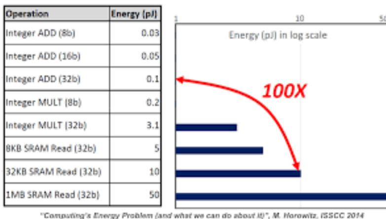
Figure 34.17. In this visualization, we can note the massive reductions in energy use by quantized operations (Isscc (2014)).
