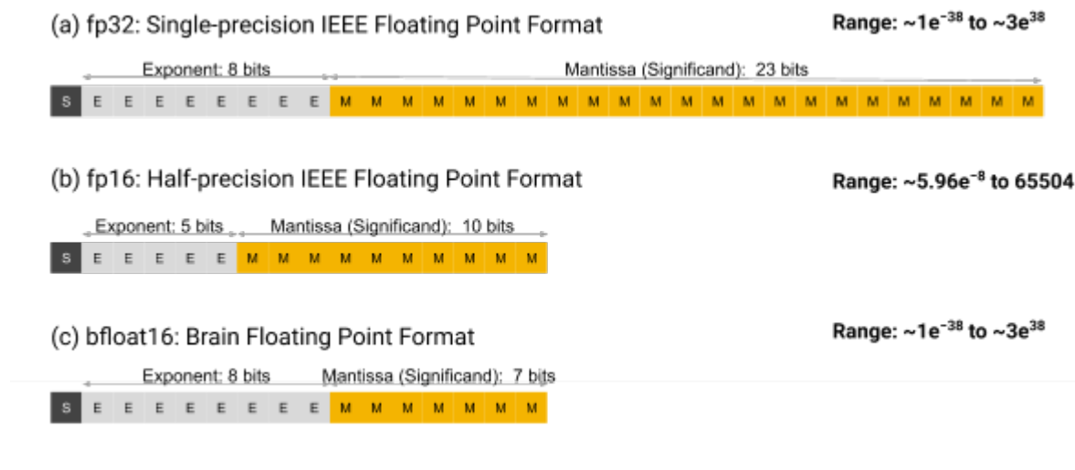
Figure 30.6. Three floating-point formats. Source: Google blog
