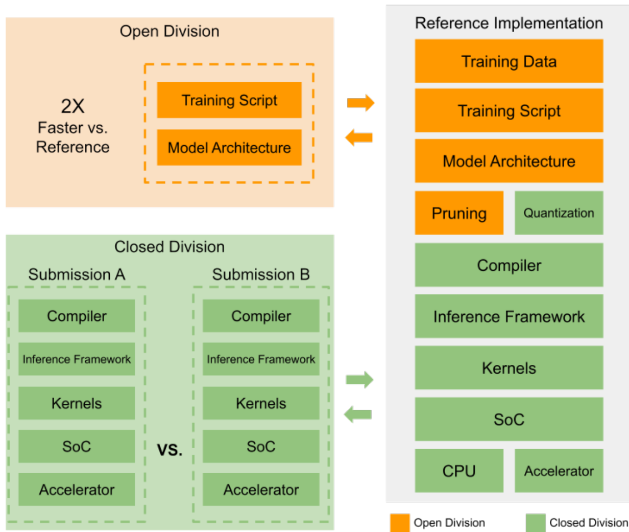
Figure 42.4. MLPerf Tiny modular design. Credit: Mattson et al. (2020a).
