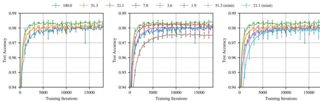
Figure 34.7. An example experiment from the lottery ticket hypothesis showing pruning and training experiments on a fully connected LeNet over a variety of pruning ratios: note the first plot showing how pruning is able to reveal a subnetwork nearly one-fifth the size that trains to a higher test accuracy faster than the unpruned network. However, further note how in the second plot that further pruned models in models that both train slower and are not able to achieve that same maximal test accuracy due to the lower number of parameters.
