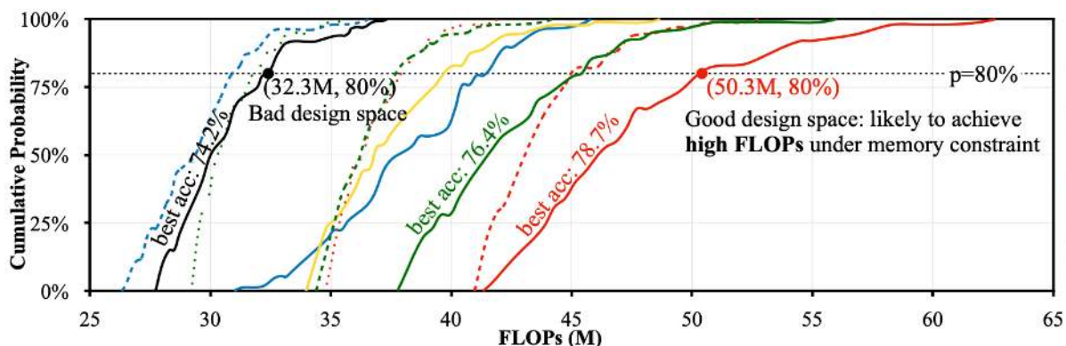
Figure 34.39. A diagram showing how search spaces with high probability of finding an architecture with large number of FLOPs provide models with higher accuracy (J. Lin et al. 2020)
