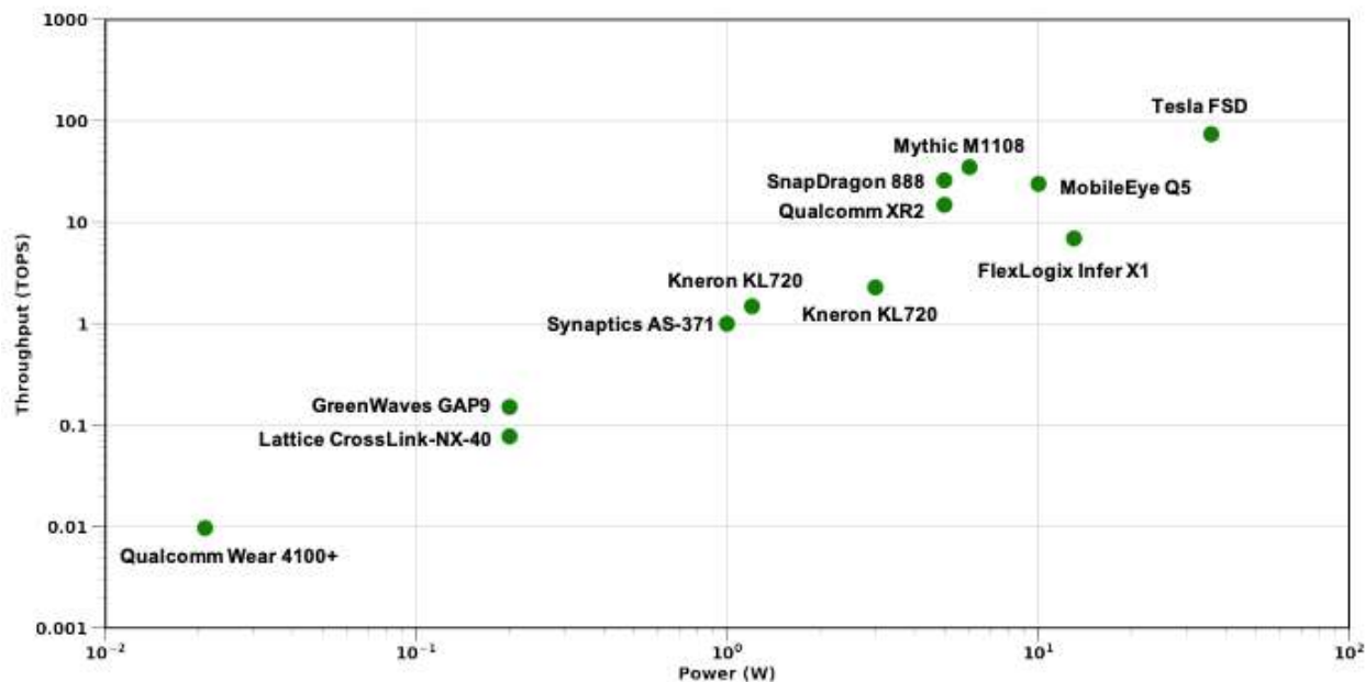
Figure 34.37. Throughput comparison of different commercial edge processors for NN inference at the edge (Gholami et al. (2021)).
