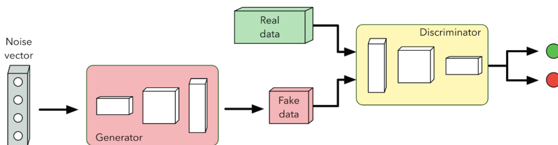
Figure 54.15. Flowchart of GANs. Credit: Rosa and Papa (2021).
