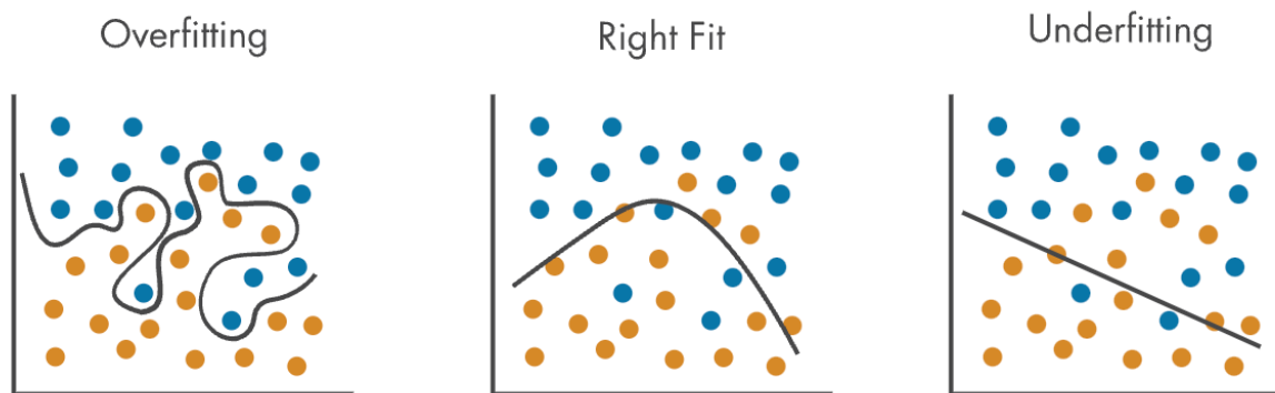
Figure 26.6. Training neural networks require striking the right balance between overfitting, and underfitting, and is a key consideration in AI training.
