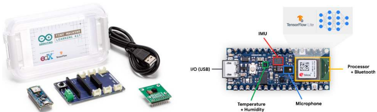
Figure 10.5. Tiny ML Example: (Left) A TinyML kit that includes Arduino Nano 33 BLE Sense, an OV7675 camera module, and TinyML shield. (Right) The Nano 33 BLE includes a host of onboard integrated sensors, a Bluetooth Low Energy module, and an Arm Cortex-M microcontroller that can run neural-network models using TensorFlow Lite for Microcontrollers. (Source: Widening Access to Applied Machine Learning with TinyML)
