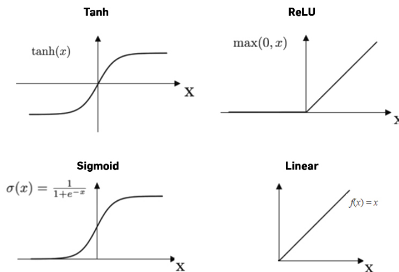
Figure 26.7. Common activation functions
